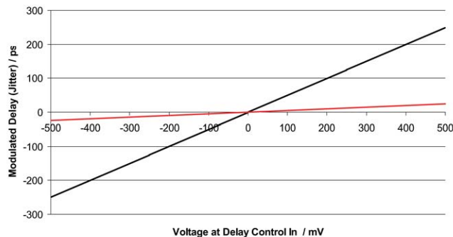
Figure 2: Modulated Delay (Jitter) vs Voltage Level at Delay-Control-Input for \pm 250\text{ps} and \pm 25\text{ps} settings
