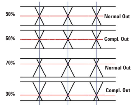
Figure 2: Variable Crossover
