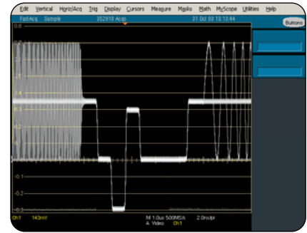
▶ Video Design. Illustration of triggering on an analog HDTV tri-level sync signal and examining horizontal blanking interval.
