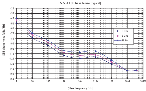
Figure 10-5. E5053A LO phase noise (typical) (0 dBm input, start offset frequency = 1 Hz, correlation = 1, measurement time = 13 sec.)
