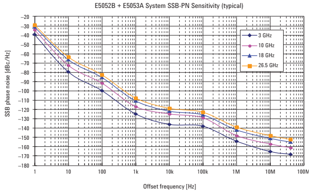
Figure 10-2. System phase noise sensitivity (E5053A + E5052B) (typical) (0 dBm input, start offset frequency = 1 Hz, correlation = 1, L.O. optimization: > 150 kHz, measurement time = 12.9 sec.)
