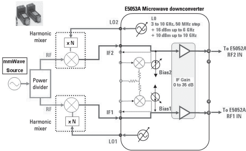
Figure 10-4. System phase noise sensitivity (E5053A + E5052B) (typical)
