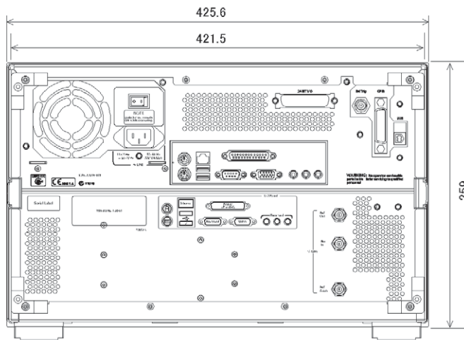
Figure 8-2. Rear view
