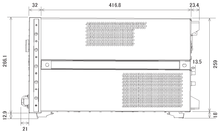
Figure 8-3. Side view
