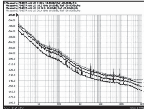
Figure 10-3. Measurement samples for the ultra-low noise N5507A LO
