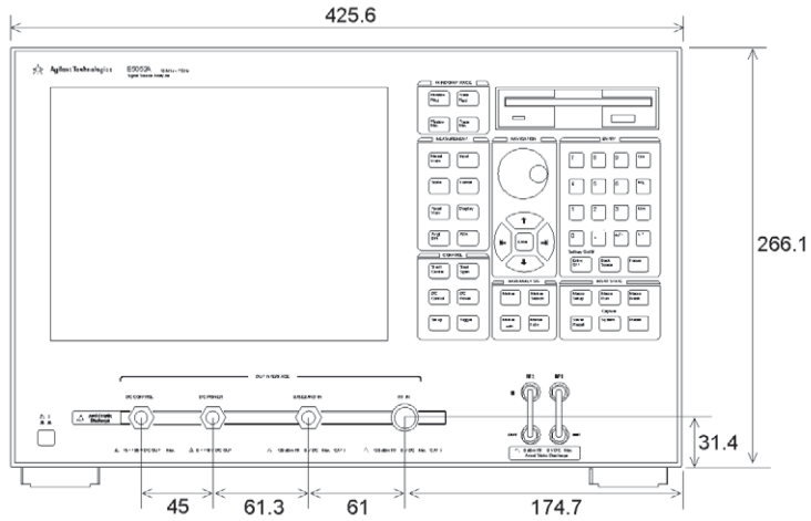
Figure 8-1. Front view
