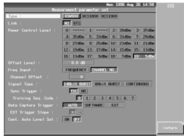
▲ GSM setting screen
