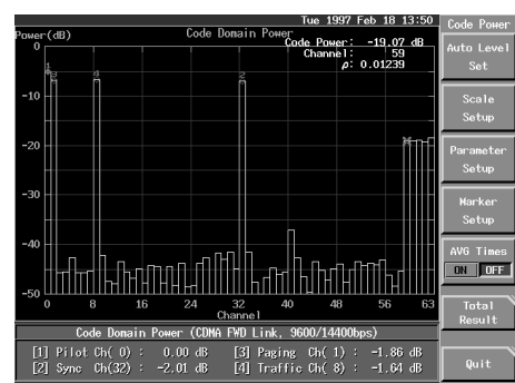
▲ CDMA code domain power measurement
