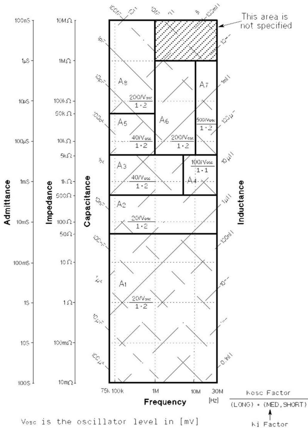
Figure 1-3. Accuracy equations, K_i factor, and K_{osc} factor (test signal level \leq 1 V_{rms} )
