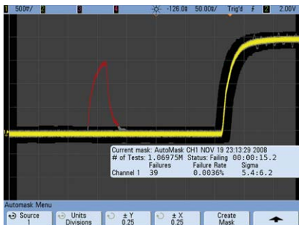
Mask testing uncovers an infrequent signal anomaly.
