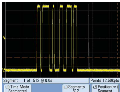
Use segmented memory to optimize available memory.
