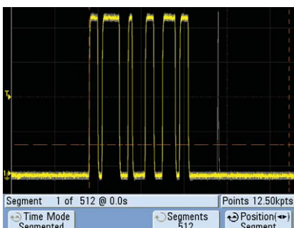
Use segmented memory to optimize available memory.
