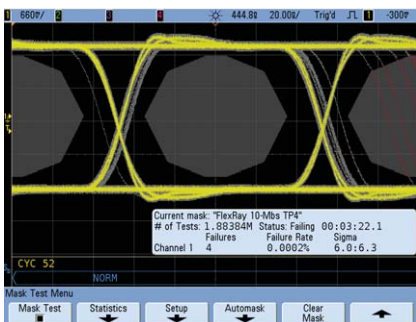
Mask testing uncovers an infrequent signal anomaly.
