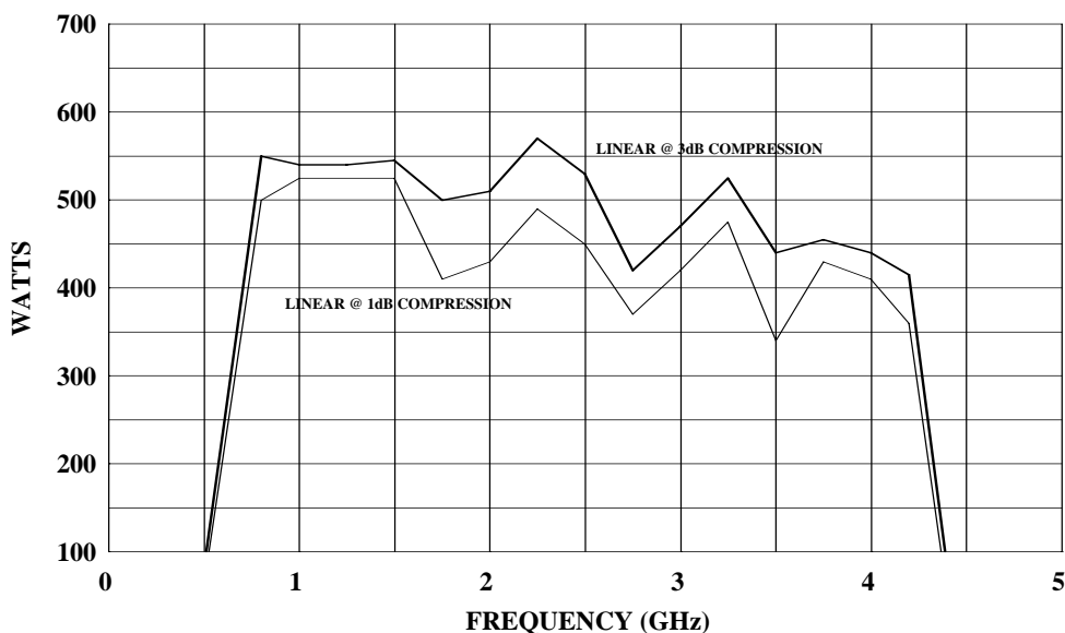
400S1G4 TYPICAL POWER OUTPUT
