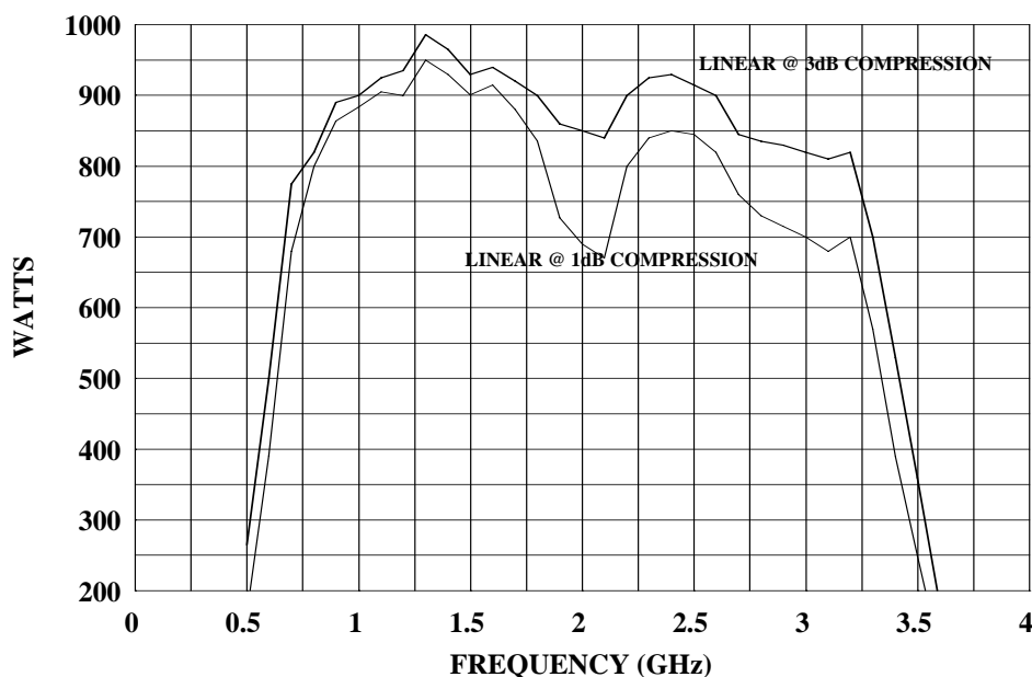
800S1G3 TYPICAL POWER OUTPUT
