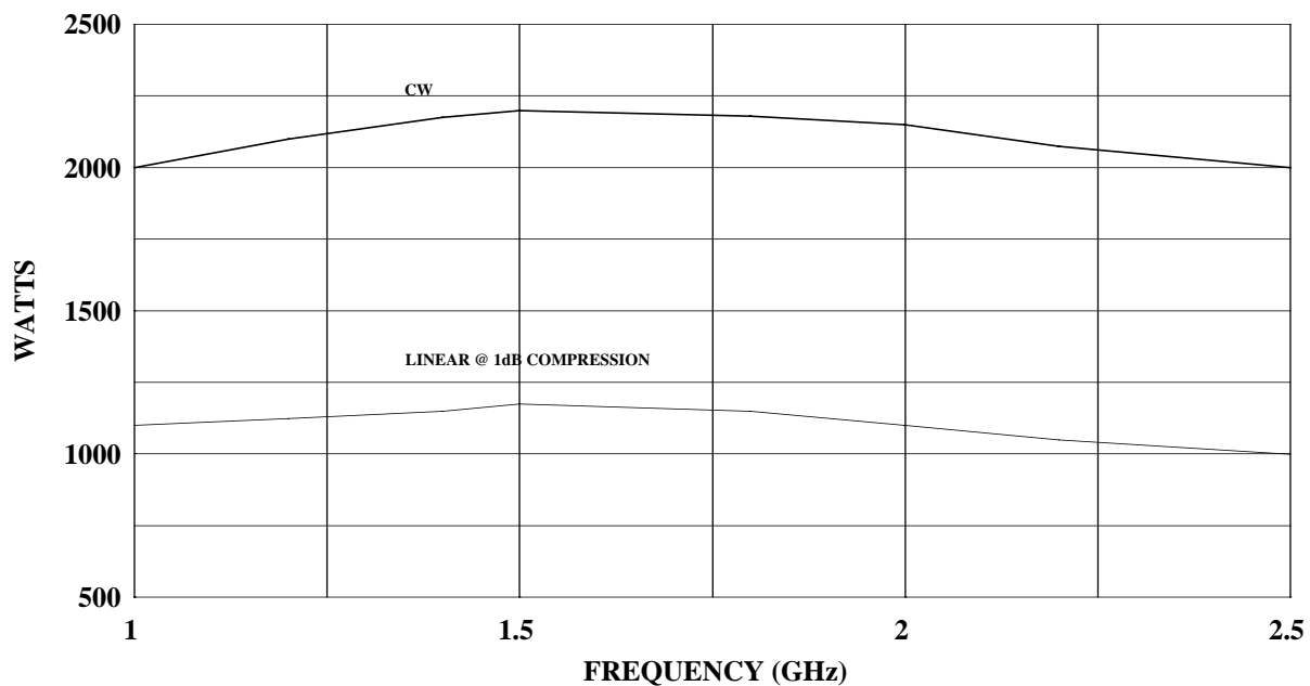
2000T1G3 TYPICAL POWER OUTPUT
