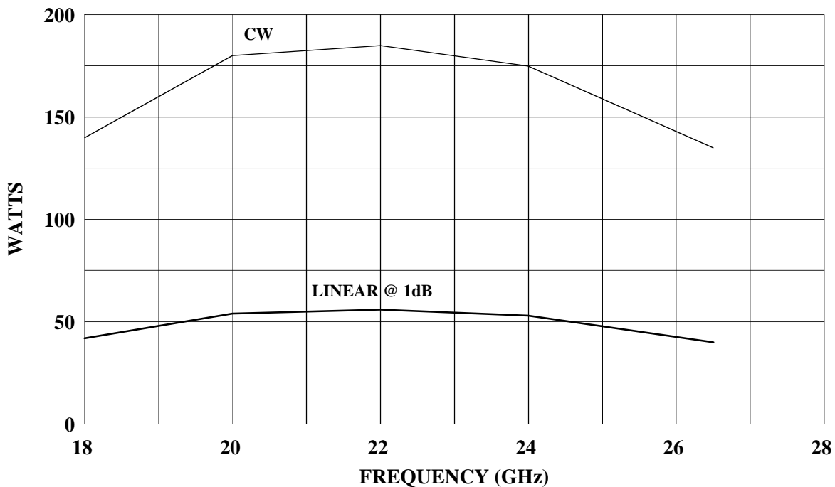
130T18G26Z5A TYPICAL POWER OUTPUT
