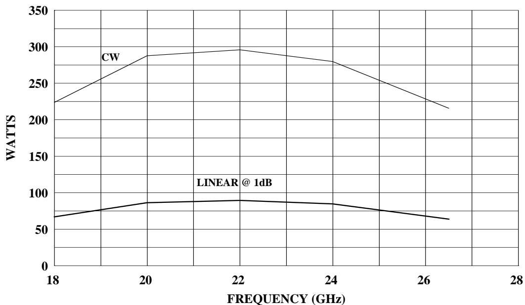
200T18G26z5 TYPICAL POWER OUTPUT
