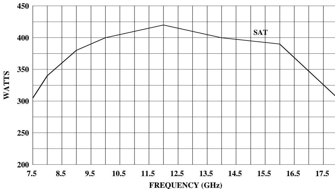
300TR7z5G18 TYPICAL POWER OUTPUT
