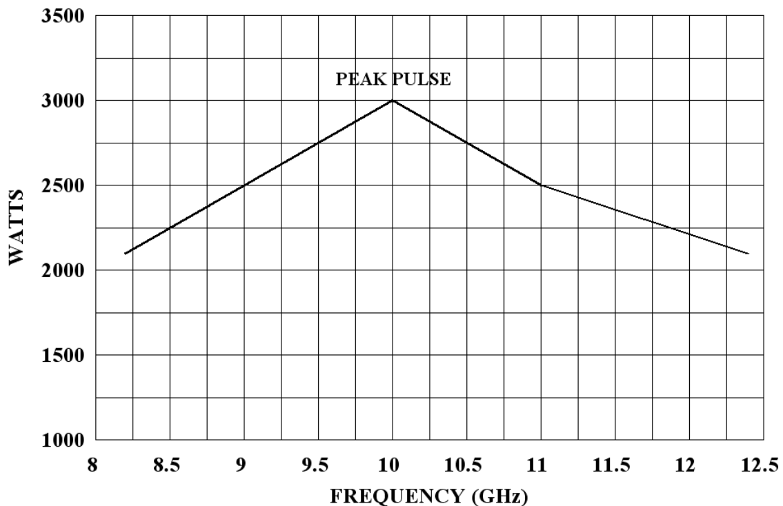
2000TP8G12 TYPICAL POWER OUTPUT
