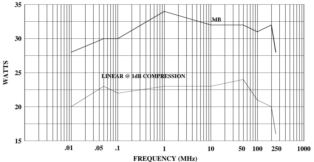
25A250A TYPICAL POWER OUTPUT
