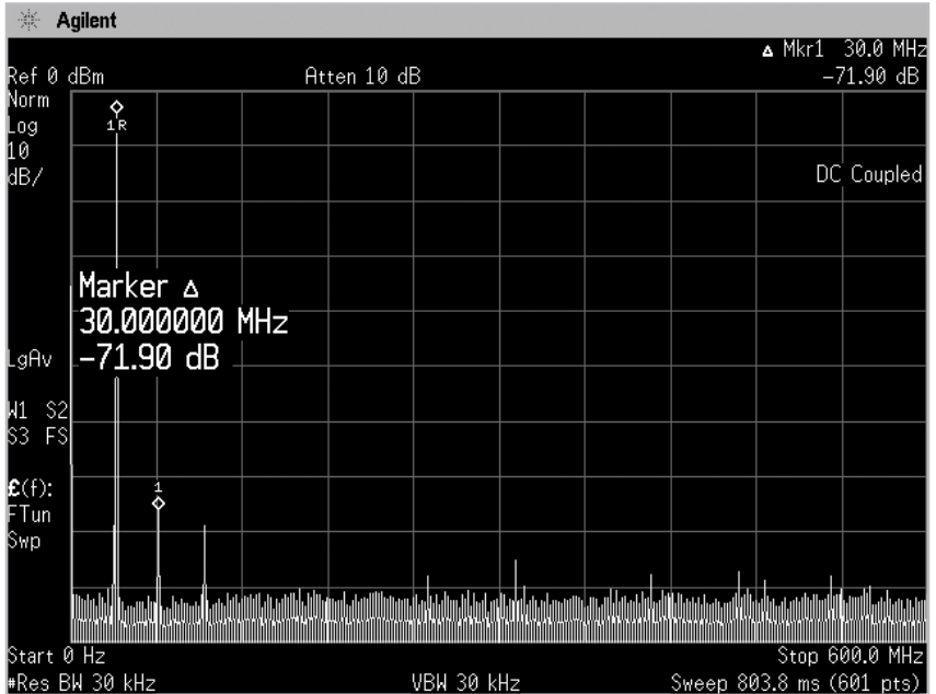
Figure 10. Spurious performance outstanding at low signal frequencies.
