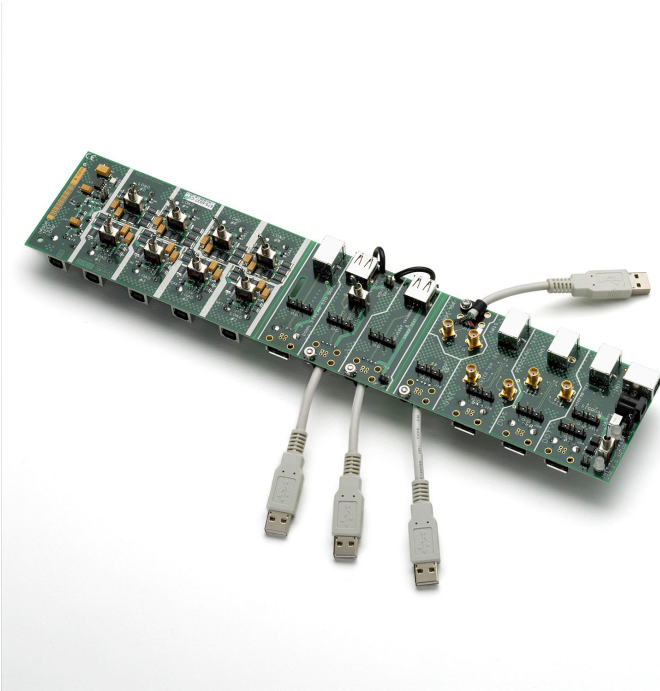
TDSUSBF USB 2.0 Test Fixture.
