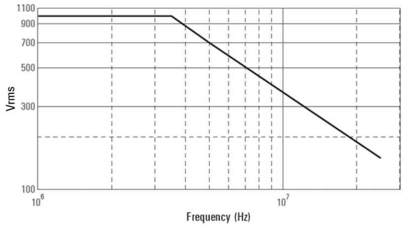
Figure 12. V_{out}/V_{in} vs. Frequency response of N2891A at 1000:1 attenuation
