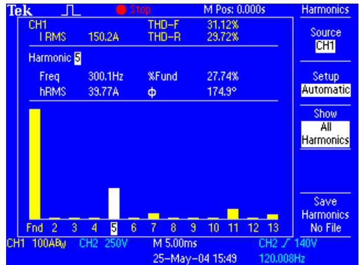
Conduct harmonic distortion measurements with TPS2PWR1 software.
