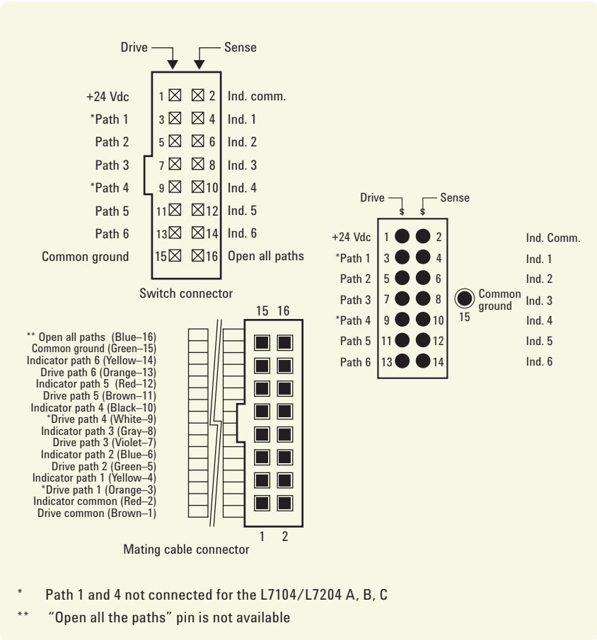
Figure 14. Drive connection diagrams with Option 100
