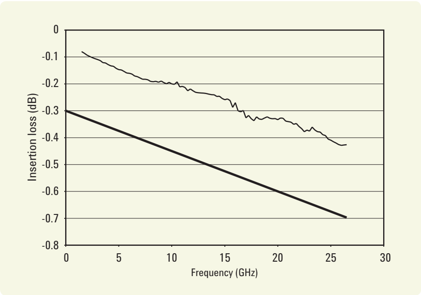
Figure 11. Agilent L Series multipoint switch insertion loss versus frequency
