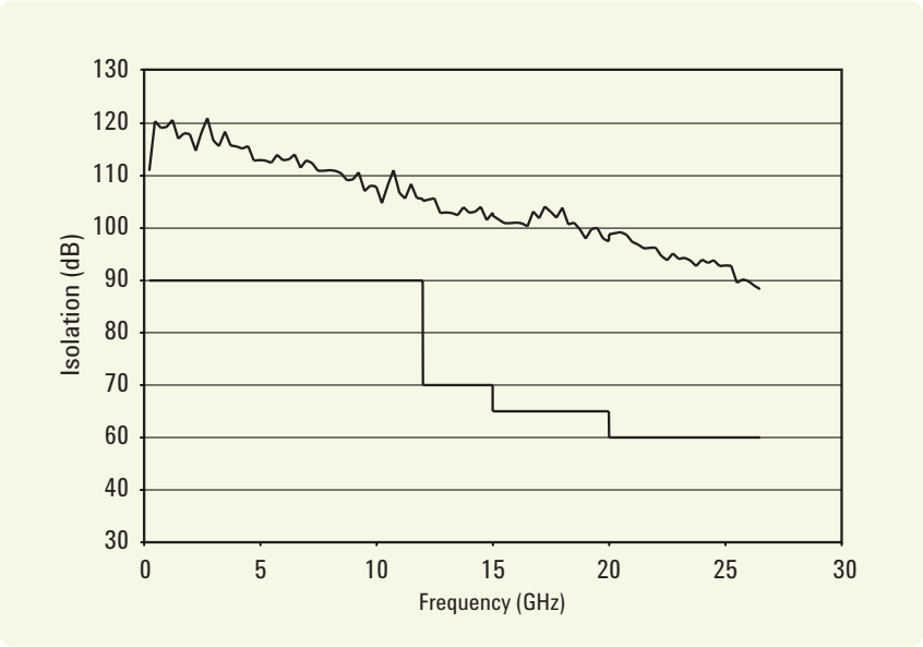
Figure 12. Agilent L Series multipoint switch isolation versus frequency
