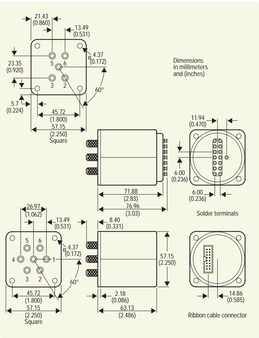
Figure 13. Product dimensions for L7104/106 A,B,C and L7204/206 A,B,C
