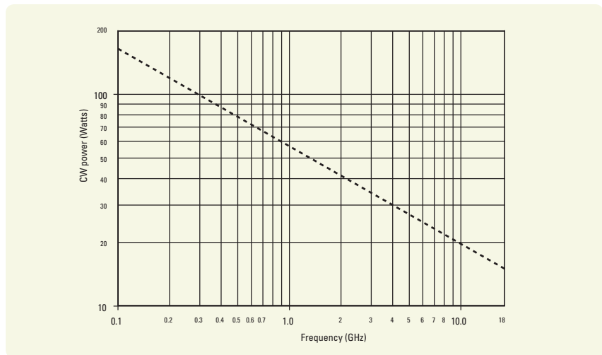
Figure 8. Power rating for cold switching at 75 °C
