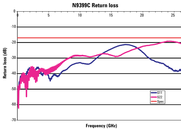
Figure 8. N9399C typical return loss versus frequency
