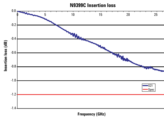
Figure 9. N9399C typical insertion loss versus frequency
