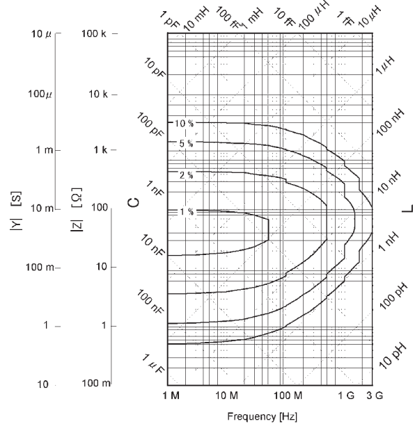
Figure 3. |Z| , |Y| Measurement accuracy when open/short/load calibration is performed. Oscillator level \geq -33 dBm. Point averaging factor \leq 7 within \pm 5 ^{\circ} C from the calibration temperature.
