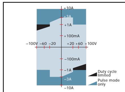
Model 2430 1kW Pulse Mode SourceMeter
