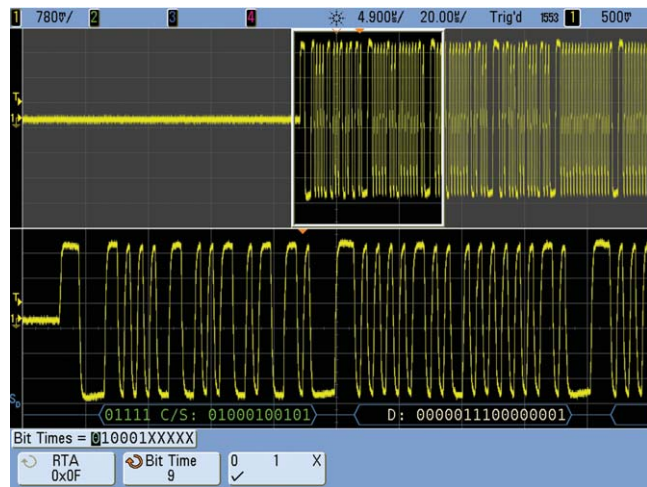
Figure 4. Triggering on a Command Word with a receive data instruction.
