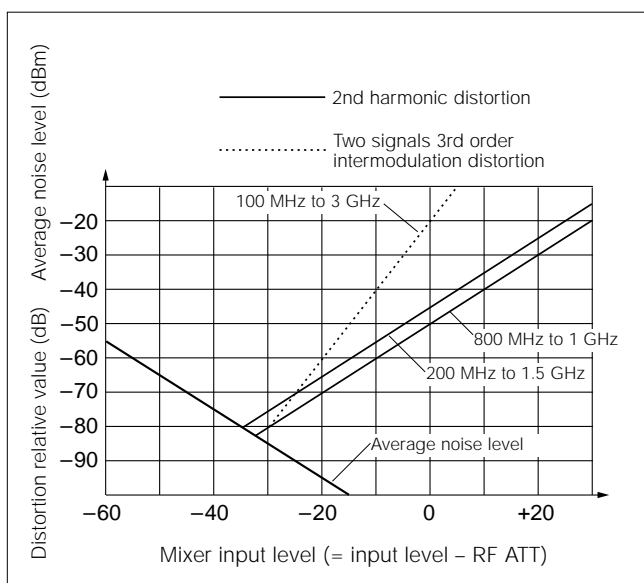
Distortion characteristics
