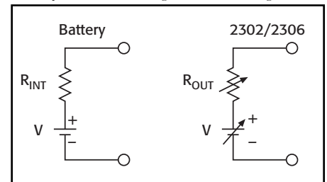
Figure 1. Simplified schematic of a battery and the 2302/2306.
