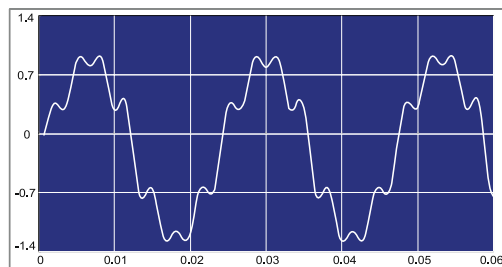
Harmonic Waveform
